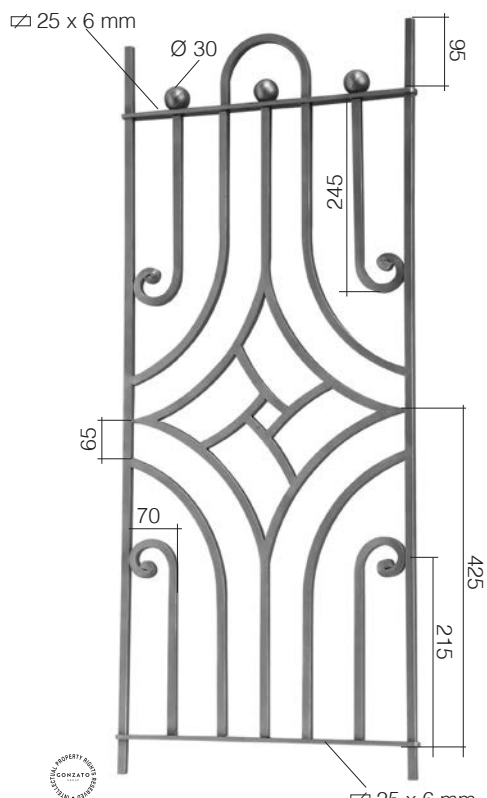
Art. GD212/1 \square 25 x 6 mm \square 12 x 12 mm 420 x 1000 mm
