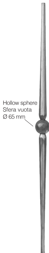
Art. 1208/5 Ø 30 mm H 900 mm
