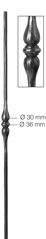
Art. 508/3/C Ø 14 mm H 1000 mm
