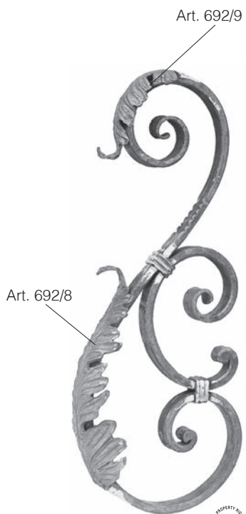
Art. 802/2 \square 25 x 12 mm H 650 mm L 270 mm
