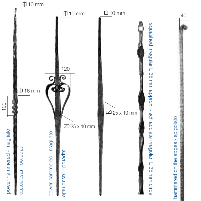
Art. 96/1 \varnothing 16 mm H 1000 mm Art. 96/3 H 900 mm Art. 96/3/S H 900 mm Art. 96/4 \varnothing 18 mm H 830 mm Art. 595/18 \varnothing 12 x 12 mm H 900 mm
