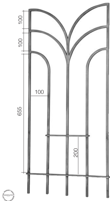
Art. GD68/1 \square 12 x 12 mm 480 x 1000 mm
