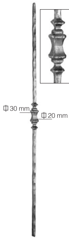
Art. 110/3 Ø 12 x 12 mm H 1000 mm
