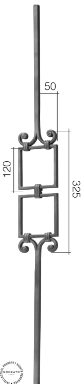
Art. GD184/1 \square 14 mm 115 x 1000 mm
