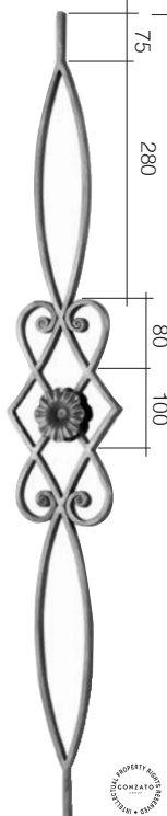
Art. GD16/1 □ 14 x 8 mm 160 x 1000 mm
