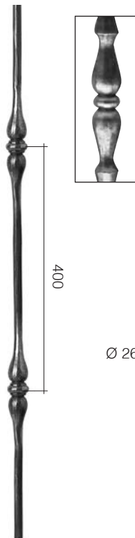
Art. 508/4/C Ø 14 mm H 1000 mm
