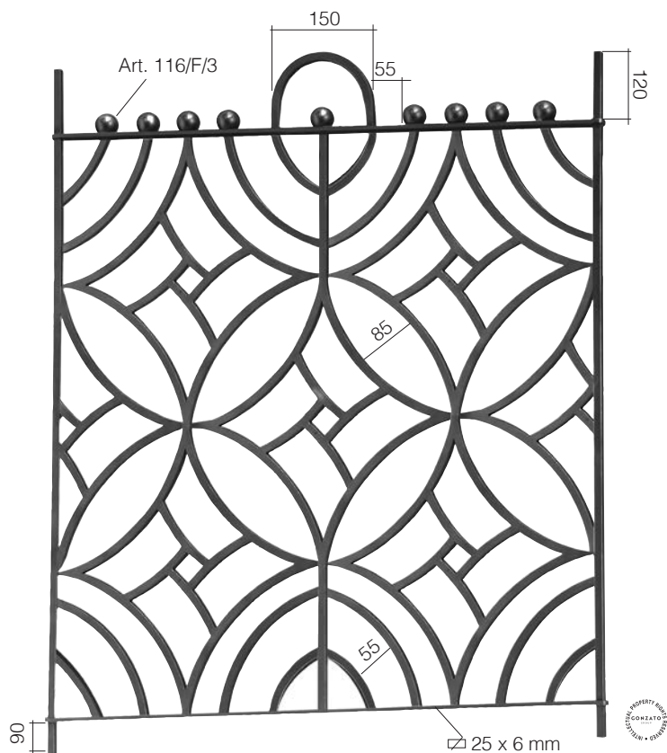
Art. GD211/1 \square 12 x 12 mm 830 x 1000 mm
