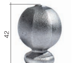
Art. 116/A/22 sfera Ø 30 mm base Ø 22 mm
