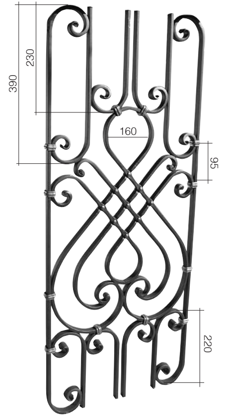
Art. GD99/1 □ 16 x 8 mm 420 x 1000 mm
