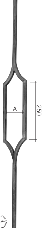
Art. GD25/3 \varnothing 14 mm 110 x 1000 mm A = 82 mm Art. GD243/2 \varnothing 12 mm 110 x 1000 mm A = 86 mm
