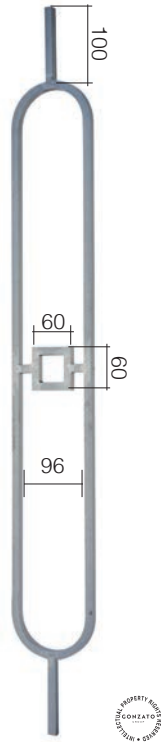
Art. GD78/6 Ø 12 mm 120 x 1000 mm
