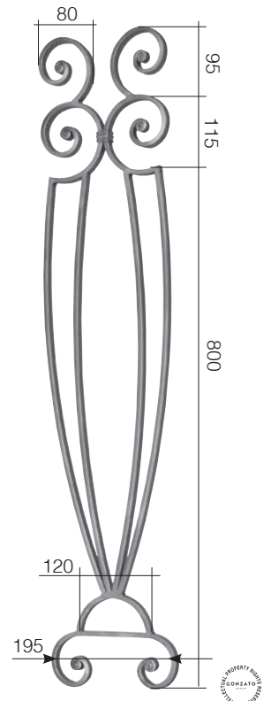
Art. GD175/7 ∅ 14 x 8 mm 200 x 1000 mm
