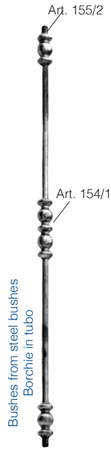
Art. 154/6 Ø 12 mm H 830 mm
