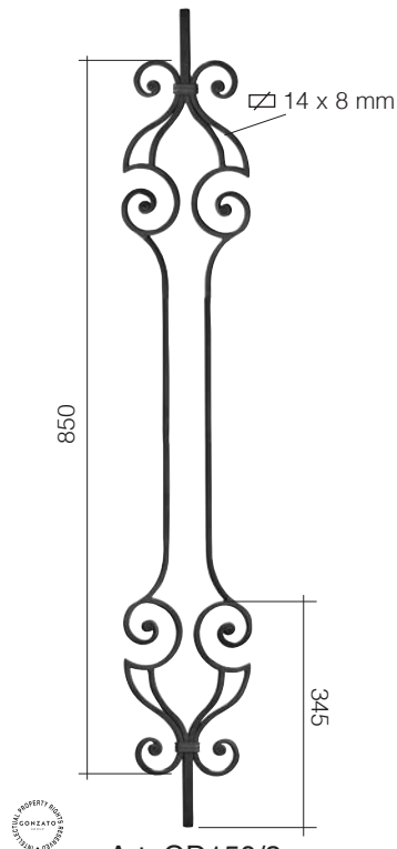
Art. GD150/2 Ø 14 x 14 mm 205 x 1000 mm
