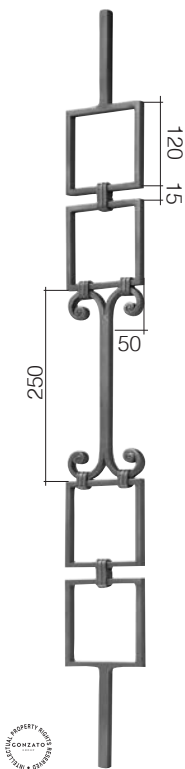
Art. GD184/2 \square 14 mm 115 x 1000 mm
