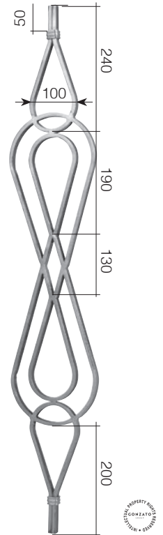
Art. GD171/1 Ø 14 x 8 mm 180 x 1000 mm
