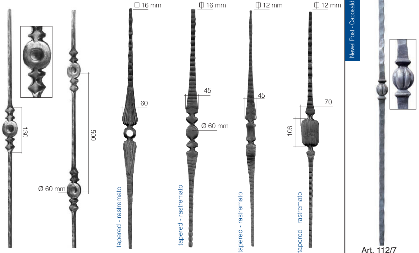
Art. 104/3 Ø 12 x 12 mm H 1000 mm
