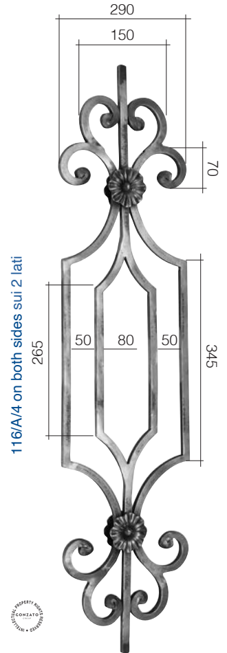
Art. GD22/1 □ 14 x 14 mm 230 x 1000 mm
