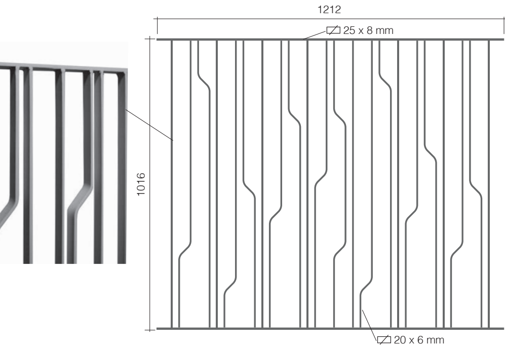
Art. GDS20FB 20 x 6 mm 1212 x 1016 mm
