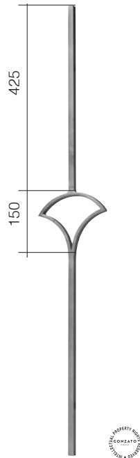
Art. GD186/1 \square 14 mm 170 x 1000 mm
