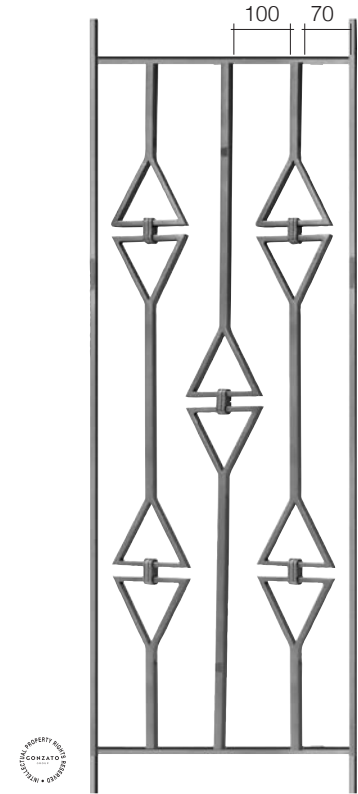
Art. GD181/3 \square 14 x 8 mm 400 x 1000 mm
