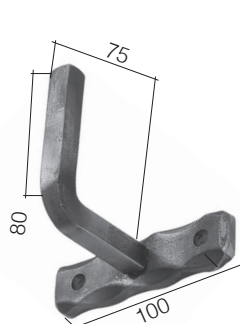
Art. 1405/1 Base 25 x 8 mm holes-foresi Ø 8,5 mm ∅ 12 x 12 mm
