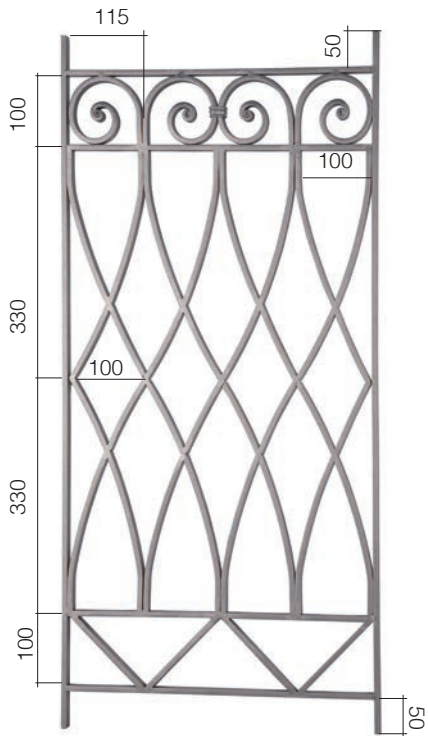
Art. GD283/1 □ 14 x 8 mm 480 x 1000 mm
