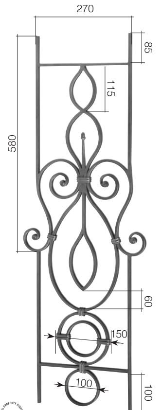
Art. GD177/2 14 x 8 mm 350 x 1000 mm
