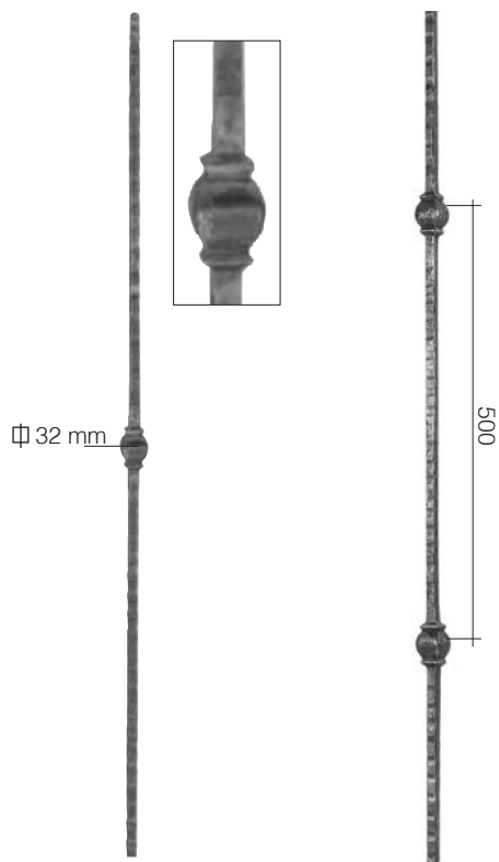
Art. 1770/8 \varnothing 12 x 12 mm H 1000 mm
