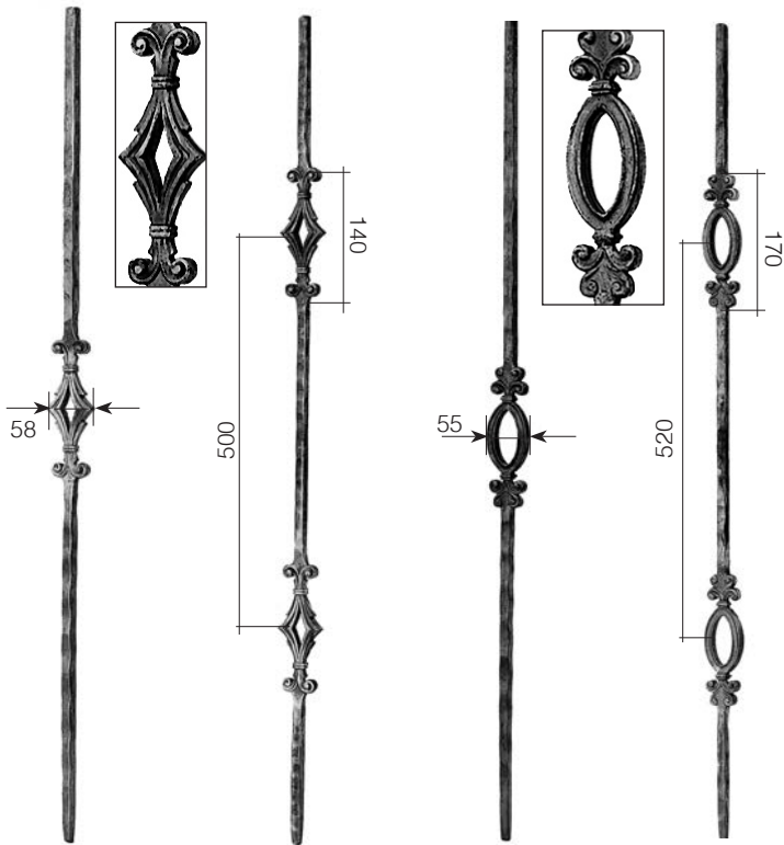
Art. 489/2 \varnothing 14 x 14 mm H 1000 mm Art. 489/1 \varnothing 14 x 14 mm H 1000 mm Art. 490/2 \varnothing 14 x 14 mm H 1000 mm Art. 490/1 \varnothing 14 x 14 mm H 1000 mm
