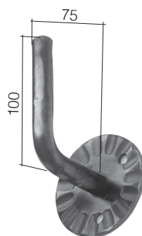
Art. 1405/3 Base Ø 80 x 4 mm holes-foresi Ø 8,5 mm Ø 16 mm
