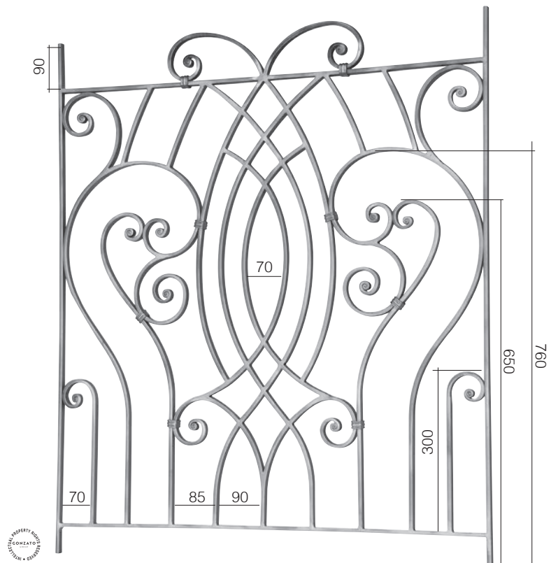
Art. GD235/1 14 x 8 mm 890 x 1000 mm
