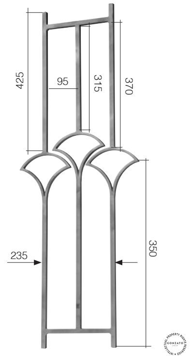
Art. GD186/3 \square 14 mm 390 x 1000 mm
