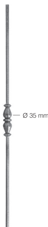
Art. 1189/3 Ø 12 mm H 900 mm
