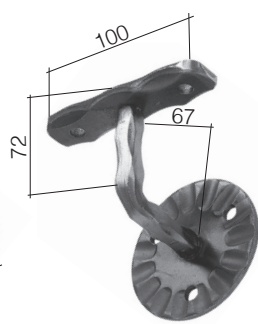
Art. 1405/2 Base Ø 80 x 4 mm holes-foresi Ø 8,5 mm ∅ 12 x 12 mm
