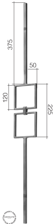
Art. GD182/1 \square 14 mm 115 x 1000 mm
