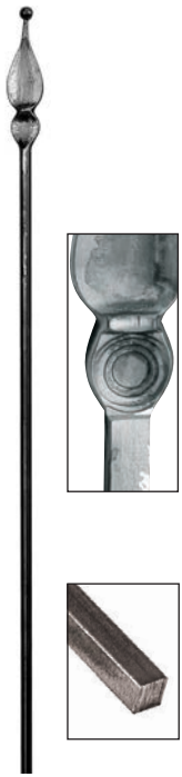
Art. 1765/15 Φ 12 x 12 mm H 1500 mm
