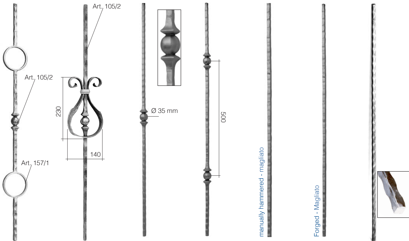
Art. 512/2 ∅ 12 x 12 mm 100 x 1000 mm
