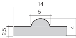
Art. 158/3 ∅ 14 x 4 mm L 4000 mm
