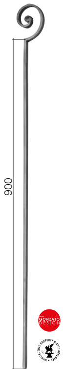
Art. GD175/6 □ 14 x 8 mm H 1000 mm L 85 mm
