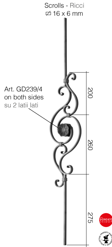
Art. GD271/5 Ø 16 x 8 mm 175 x 1000 mm
