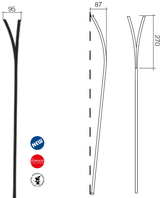
Art. GD290/2 Ø 12 mm H 1000 mm
