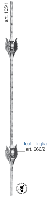
Art. 492/1 Ø 12 x 12 mm H 1000 mm
