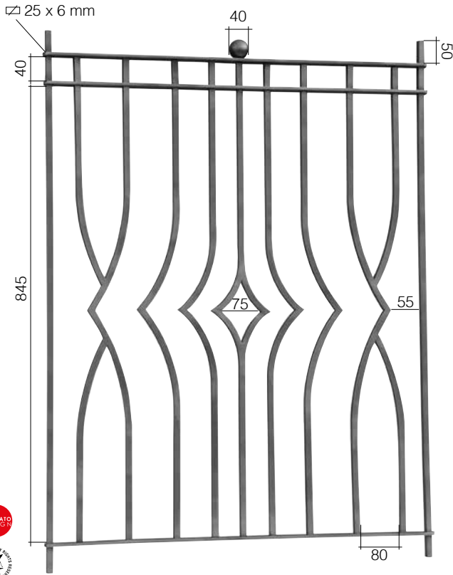
Art. GD232/1 ⌀ 12 x 12 mm 740 x 1000 mm
