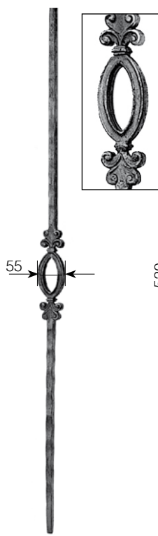
Art. 490/2 Ø 14 x 14 mm H 1000 mm
