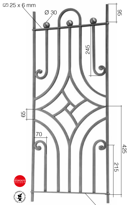
Art. GD212/1 □ 25 x 6 mm □ 12 x 12 mm 420 x 1000 mm
