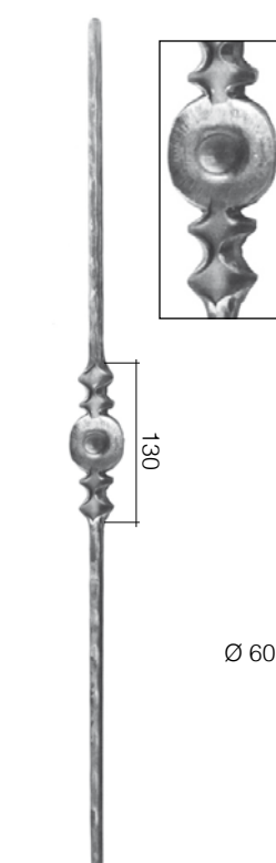
Art. 104/3 Ø 12 x 12 mm H 1000 mm
