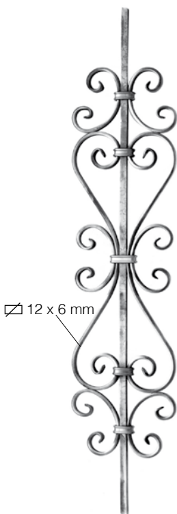
Art. 52/E/2 Ø 12 x 12 mm 185 x 900 mm
