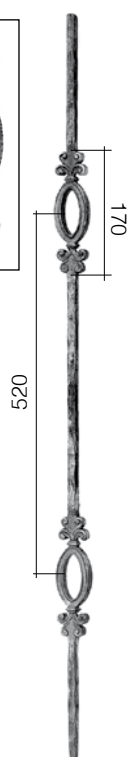
Art. 490/1 Ø 14 x 14 mm H 1000 mm
