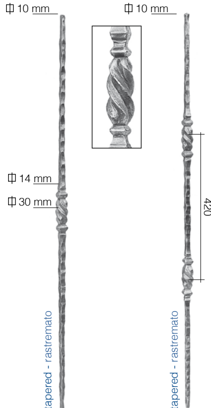
Art. 505/3 Ø 14 x 14 mm H 1000 mm Art. 505/4 Ø 14 x 14 mm H 1000 mm
