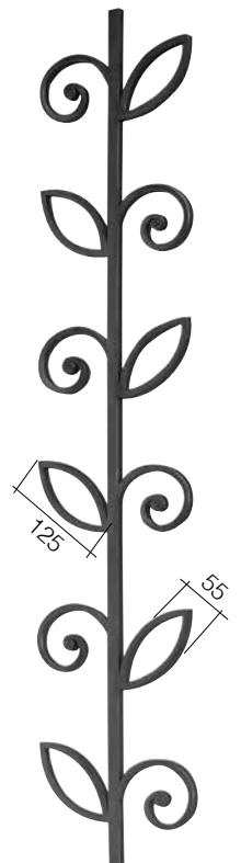
Art. GD176/3 ∅ 14 x 14 mm 200 x 1000 mm
