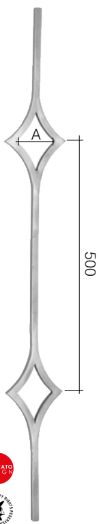
Art. GD25/1 ∅ 14 mm 120 x 1000 mm A = 75 mm Art. GD58/2 ∅ 12 mm 120 x 1000 mm A = 80 mm
