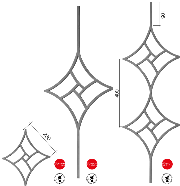
Art. GD211/2 □ 12 mm 395 x 395 mm
