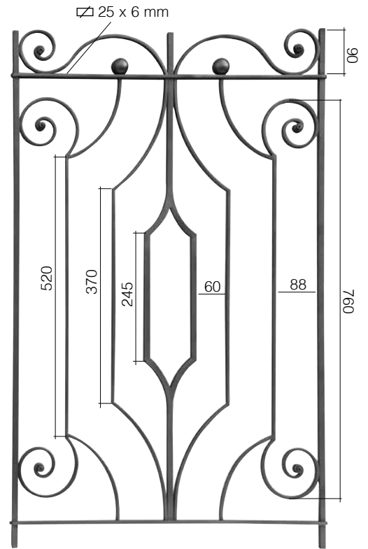
Art. GD242/1 ⌀ 12 x 12 mm 640 x 1000 mm
