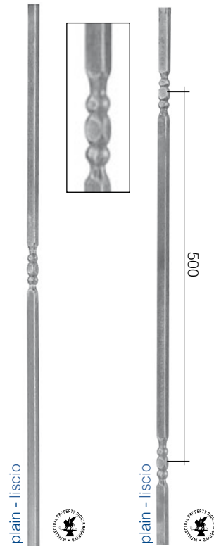
Art. 1773/6 Ø 12 x 12 mm H 1000 mm Art. 1773/5 Ø 12 x 12 mm H 1000 mm Art. 1773/2 Ø 14 x 14 mm H 1000 mm Art. 1773/1 Ø 14 x 14 mm H 1000 mm
