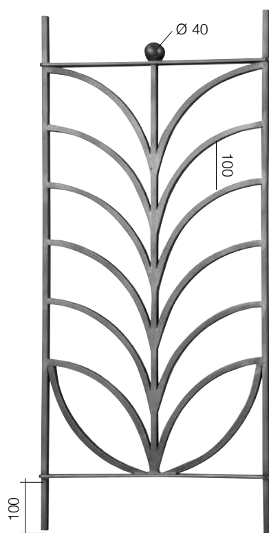
Art. GD73/1 Ø 12 x 12 mm 455 x 1000 mm
