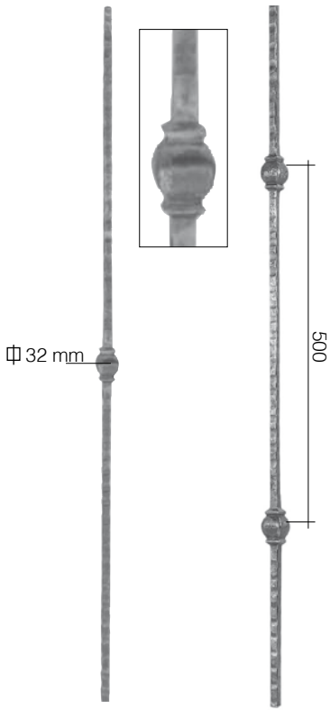
Art. 1770/8 Ø 12 x 12 mm H 1000 mm Art. 1771/8 Ø 12 x 12 mm H 1000 mm
