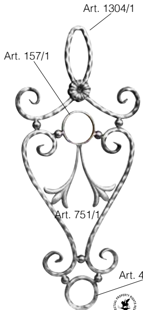
Art. 475/1 hammered - spigolato ∅ 12 x 12 mm 380 x 825 mm
