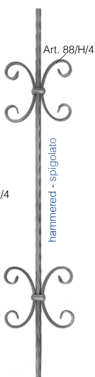
Art. 584/7 Ø 12 x 12 mm 165 x 900 mm
