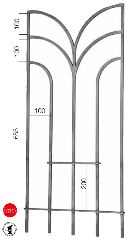
Art. GD68/1 □ 12 x 12 mm 480 x 1000 mm
