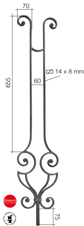
Art. GD148/1 Ø 14 x 14 mm 205 x 1000 mm
