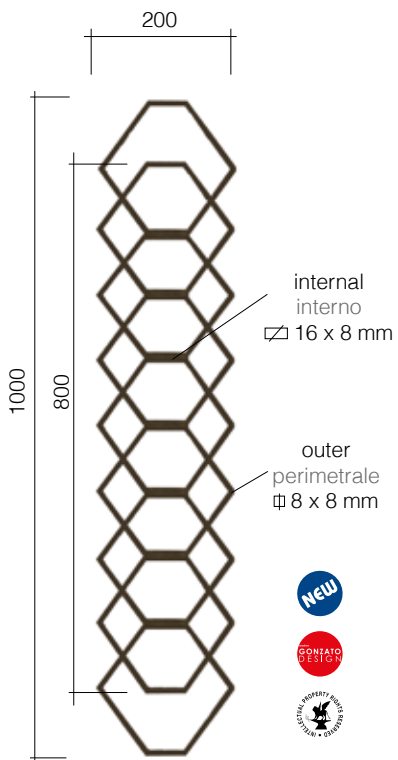
Art. GD299/3 \Phi 8 \times 8 \text{ mm} + \square 16 \times 8 \text{ mm} 200 x 1000 mm
