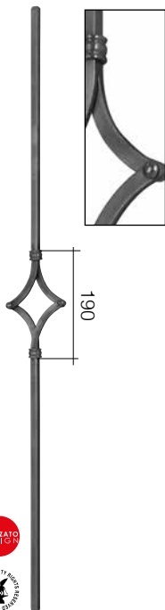
Art. GD20/1 BEST PRICE \varnothing 12 mm 110 x 1000 mm
