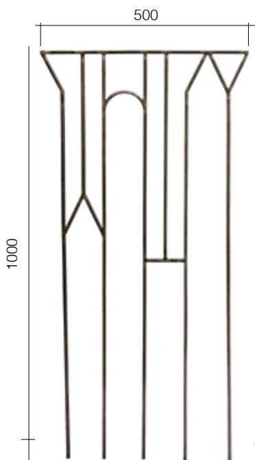
Art. GD295/1 □ 14 x 8 mm 500 x 1000 mm
