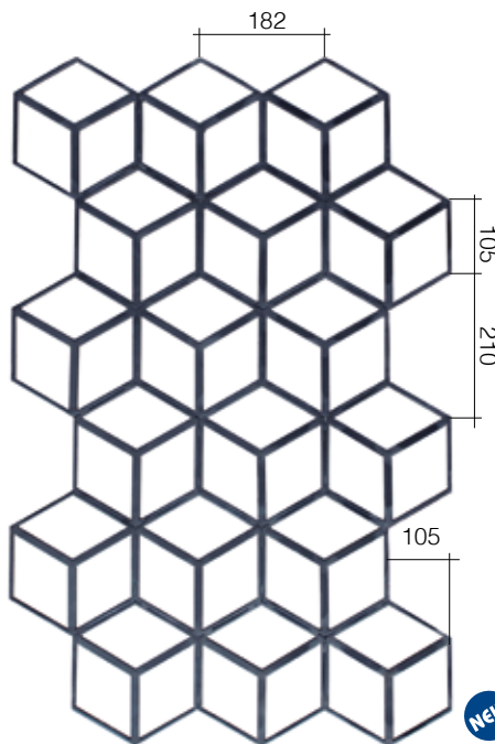
Art. GD287/4 12 \times 6 \text{ mm} + \varnothing 12 \text{ mm} 638 x 1000 mm
