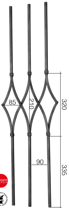
Art. GD21/1 \square 12 mm 315 x 1000 mm
