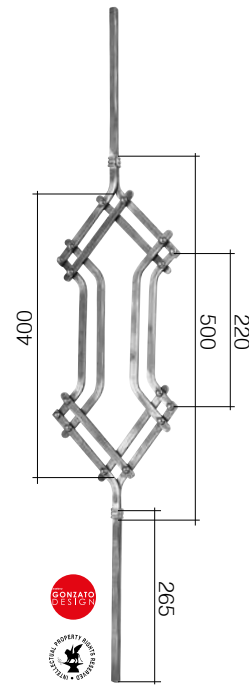
Art. GD21/5 \square 12 mm 200 x 1000 mm
