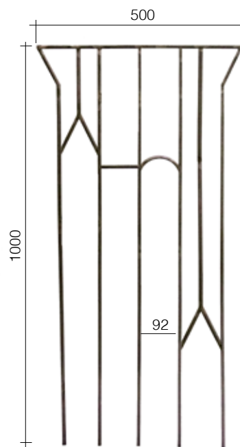
Art. GD295/2 □ 14 x 8 mm 500 x 1000 mm
