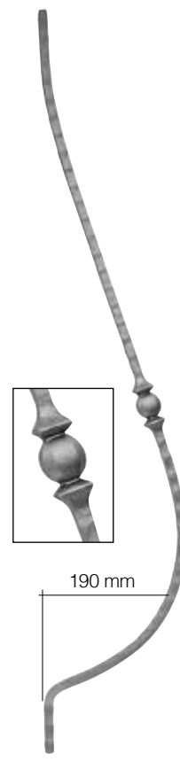
Art. 1783/5 \varnothing 12 x 12 mm H 1000 mm
