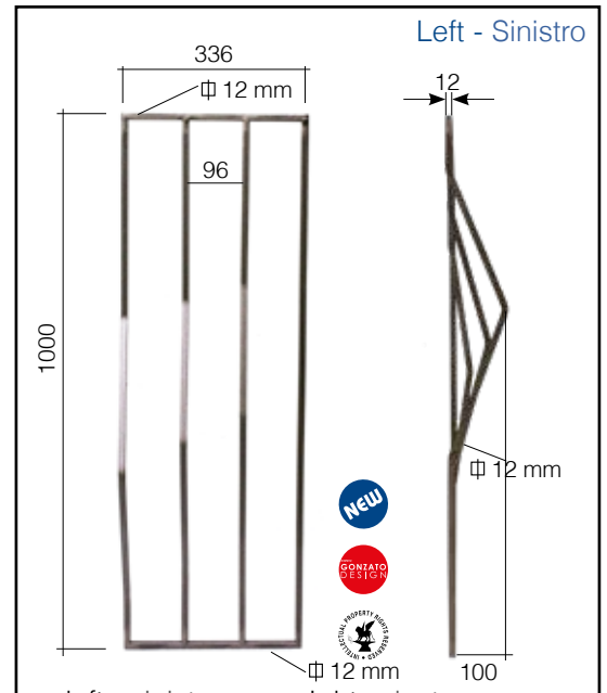
left - sinistro Art. GD293/3 12 x 12 mm 336 x 1000 mm
