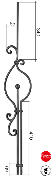
Art. GD39/3 Ø 12 mm 190 x 1000 mm
