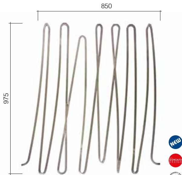
Art. GD300/1 ∅ 12 x 12 mm 850 x 975 mm
