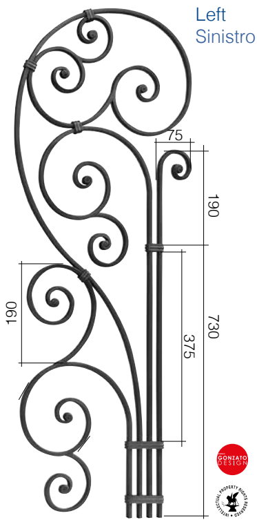
left - sinistro Art. GD164/1 Ø 14 x 8 mm L 380 mm H 1000 mm
