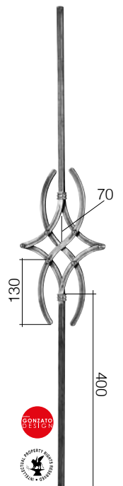
Art. GD21/6 \square 12 mm 200 x 1000 mm
