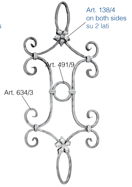
Art. 479/2 ∅ 12 x 12 mm 385 x 900 mm
