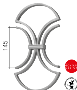
Art. GD187/2 ∅ 14 x 8 mm 190 x 325 mm
