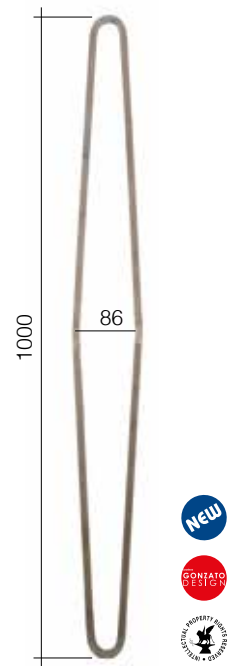
Art. GD293/2 Ø 12 x 12 mm 110 x 1000 mm
