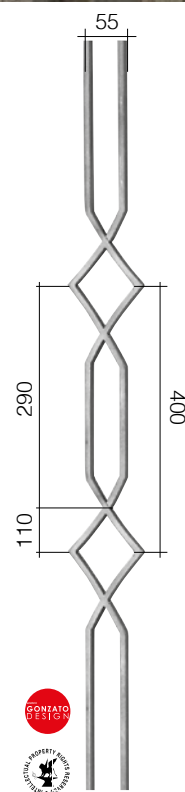
Art. GD19/2 ∅ 14 x 8 mm 100 x 1000 mm
