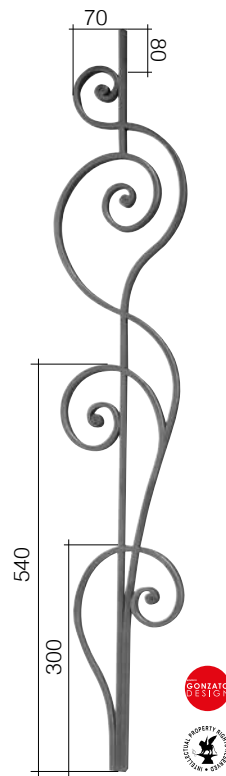
Art. GD228/2 Ø 14 x 8 mm 190 x 1000 mm
