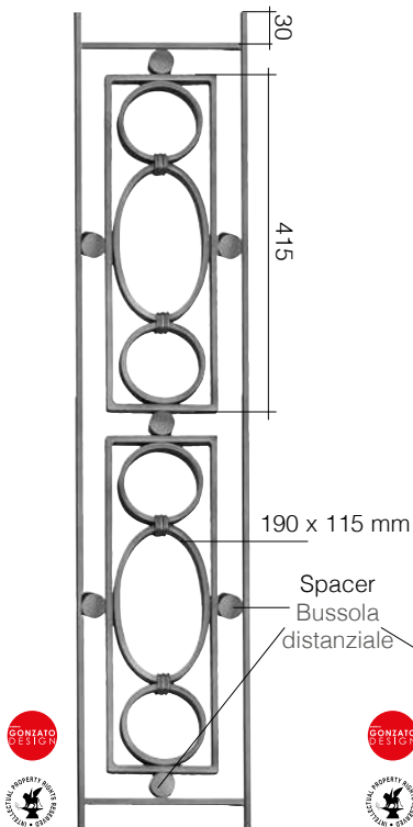
Art. GD205/2 \square 14 x 8 mm 210 x 1000 mm
