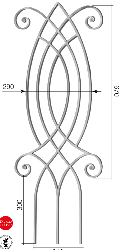
Art. GD234/1 14 x 8 mm 380 x 1000 mm
