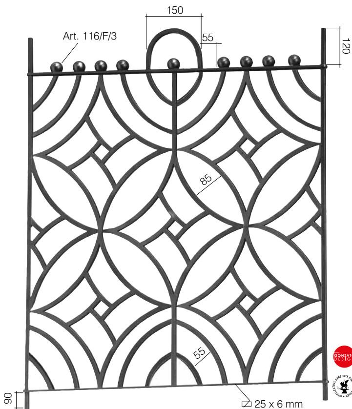
Art. GD211/1 □ 12 x 12 mm 830 x 1000 mm
