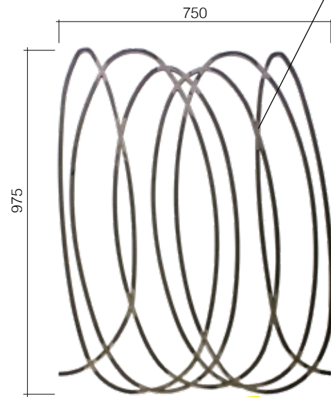
Art. GD300/2 ∅ 12 x 12 mm 750 x 975 mm
