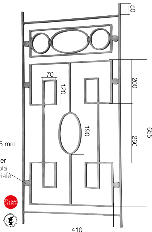
Art. GD205/1 \square 14 x 8 mm 495 x 1000 mm
