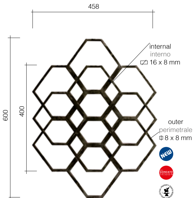
Art. GD299/4 \Phi 8 \times 8 \text{ mm} + \square 16 \times 8 \text{ mm} 458 x 600 mm
