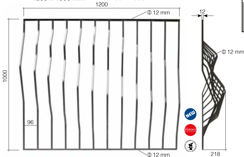
left - sinistro Art. GD289/1 12 x 12 mm 1200 x 1000 mm
