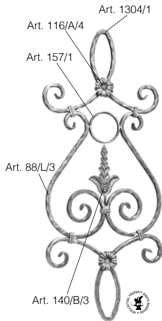
Art. 475/2 hammered - spigolato ∅ 12 x 12 mm 380 x 900 mm
