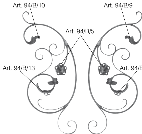
right - destro Art. 94/F/6 Ø 12 mm 420 x 970 mm
