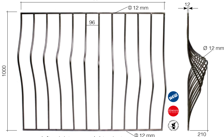
left - sinistro Art. GD294/1 right - destro Art. GD294/1/S Ø 12 mm Ø 12 mm 1200 x 1000 mm 1200 x 1000 mm
