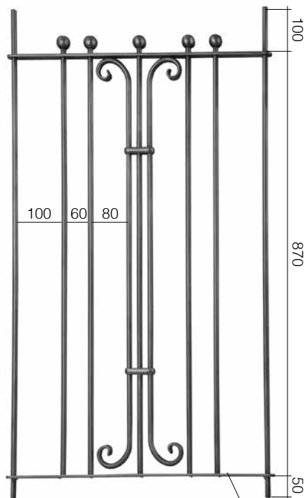
Spheres - Sfere Ø 30 mm
