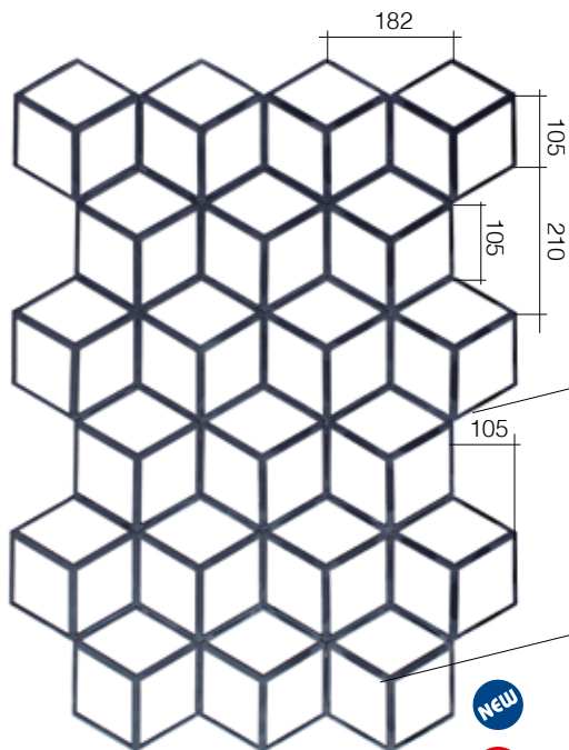
Art. GD287/1 12 \times 6 \text{ mm} + \varnothing 12 \text{ mm} 729 x 1000 mm
