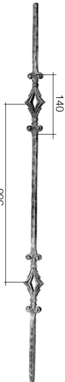
Art. 489/1 Ø 14 x 14 mm H 1000 mm
