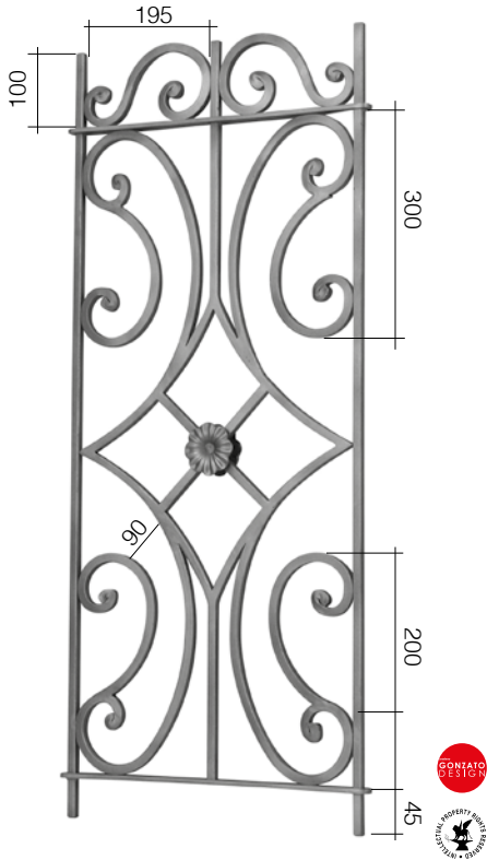
Art. GD61/1 Ø 12 x 12 mm 430 x 1000 mm
