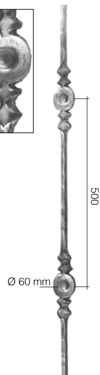
Art. 104/4 Ø 12 x 12 mm H 1000 mm
