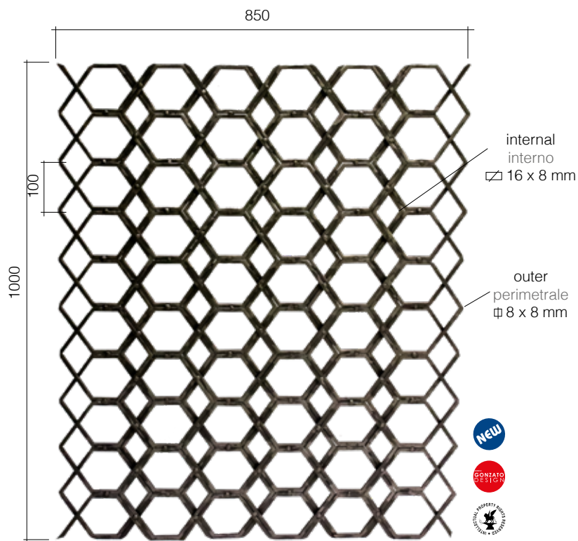
Art. GD299/1 \Phi 8 \times 8 \text{ mm} + \square 16 \times 8 \text{ mm} 850 x 1000 mm
