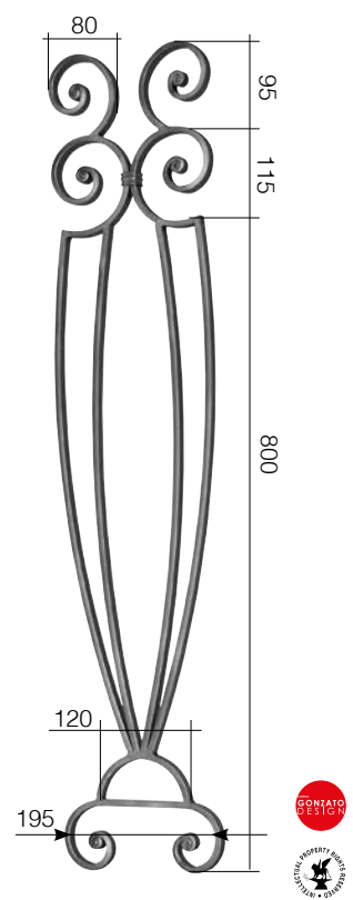
Art. GD175/7 ∅ 14 x 8 mm 200 x 1000 mm
