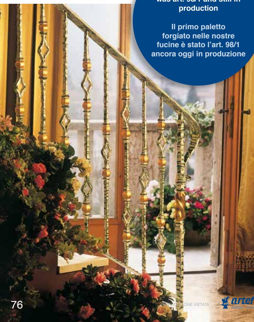
Art. 507/1 Ø 30 mm H 1000 mm
