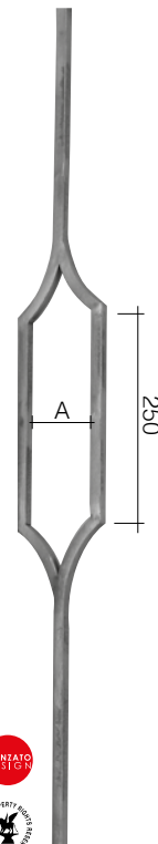
Art. GD25/3 ∅ 14 mm 110 x 1000 mm A = 82 mm Art. GD243/2 ∅ 12 mm 110 x 1000 mm A = 86 mm
