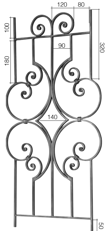
Art. GD219/1 □ 14 x 8 mm 500 x 1000 mm
