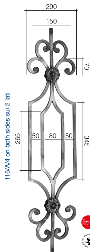
Art. GD22/1 □ 14 x 14 mm 230 x 1000 mm
