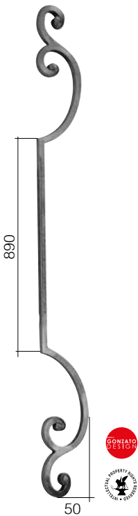
Art. GD22/3 Φ 14 x 14 mm 110 x 1000 mm
