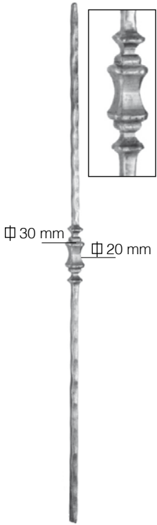
Art. 110/3 Ø 12 x 12 mm H 1000 mm
