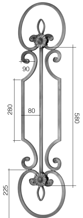
Art. GD31/2 ⌀ 14 x 14 mm 245 x 1000 mm
