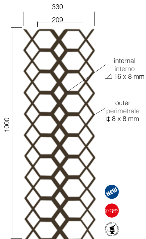
Art. GD299/2 \Phi 8 \times 8 \text{ mm} + \square 16 \times 8 \text{ mm} 330 x 1000 mm
